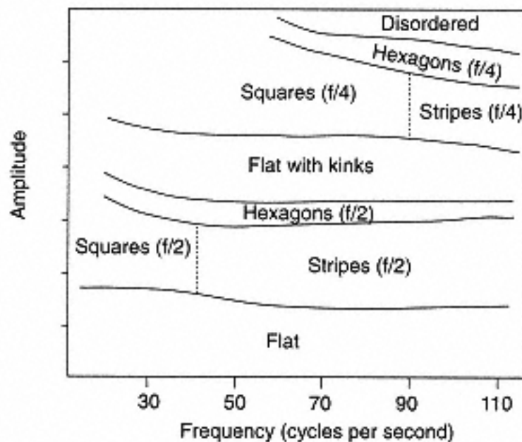
Fig. 8.4 Transitions between different wave patterns in a granular layer can be induced by altering the shaking frequency ( f ) or amplitude. (After: Umbanhowar et al. 1997.)
