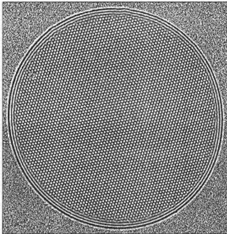
Fig. 7.10 Convection rolls can become twisted and fragmented into disordered patterns that are constantly changing in time. (Image: David Cannell.)
