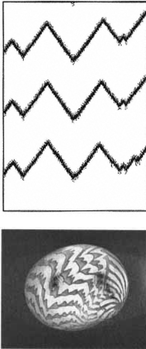
Fig. 4.20 Annihilation between travelling waves in an activator inhibitor model leads to V-shaped patterns(a), as seen on the shell of Lioconcha lorenziana (b). (Photo: Hans Meinhardt.)
