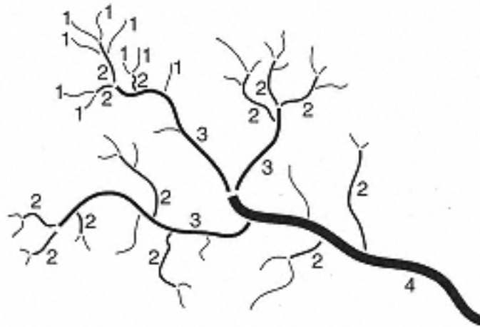
Fig. 6.19 The hierarchy of river network elements in Strahler's modification of Horton's classification scheme. Each branch is assigned an order that increases downstream.
