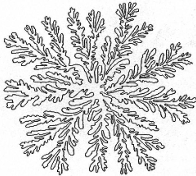
Fig. 5.15 Viscous fingering has a characteristic length scale, which determines the minimum width of the branches. So the fingers are fatter than the fine filaments of DLA clusters. (Image: Yves Couder, Ecole Normale Supérieure, Paris.)
