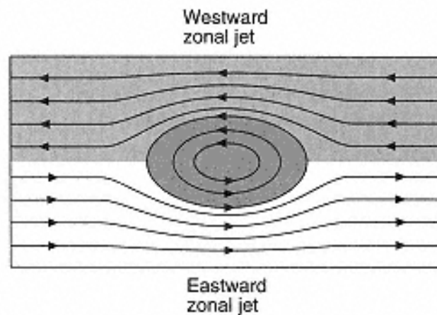
Fig. 7.47 Jupiter's Great Red Spot circulates between oppositely directed zonal jets that encircle the planet.
