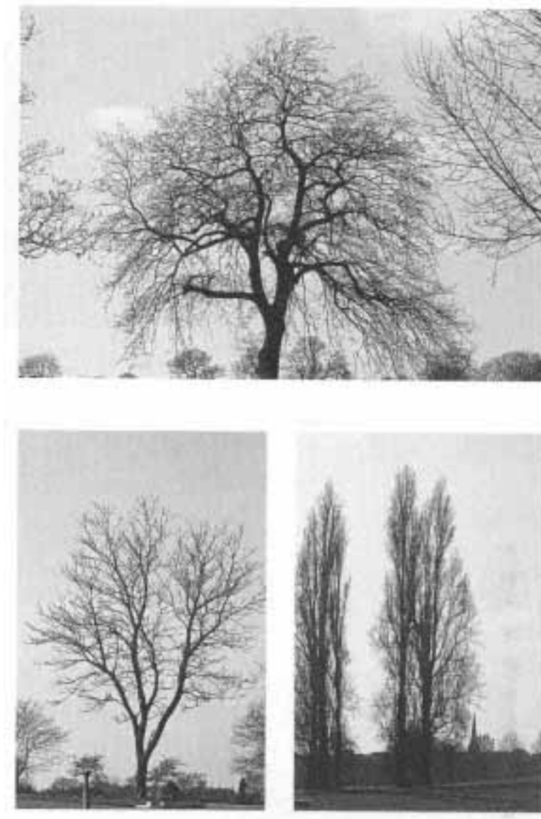
Fig. 5.3 The branching patterns of trees are often characteristic of their species.
